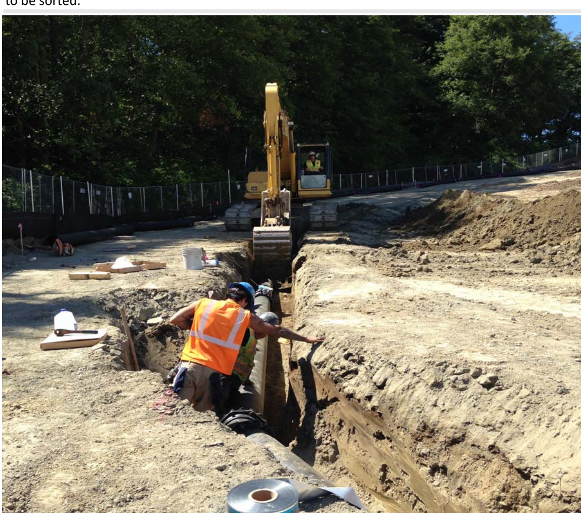
7/10/18 Laying ductile iron pipe for the fire loop.
